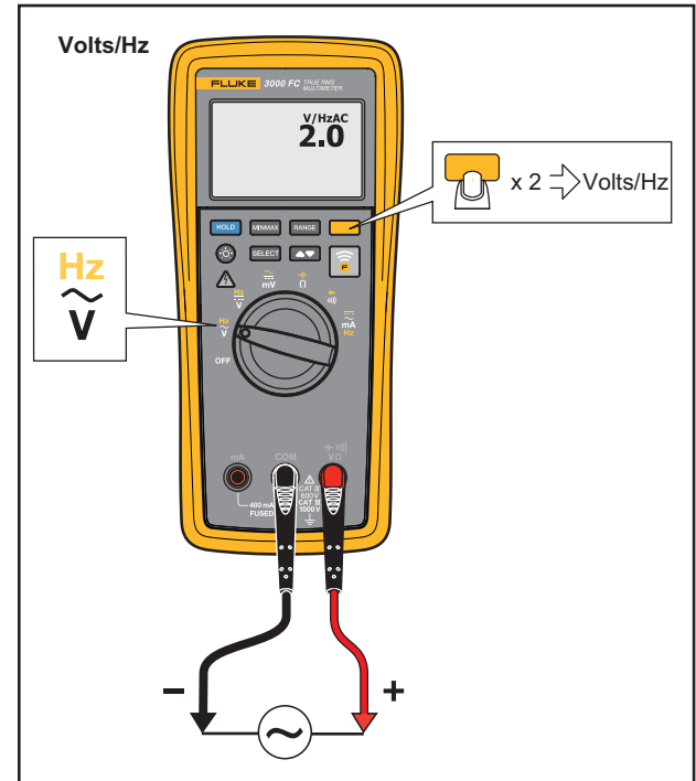
Figure 2. Ratio Volts/Hertz
